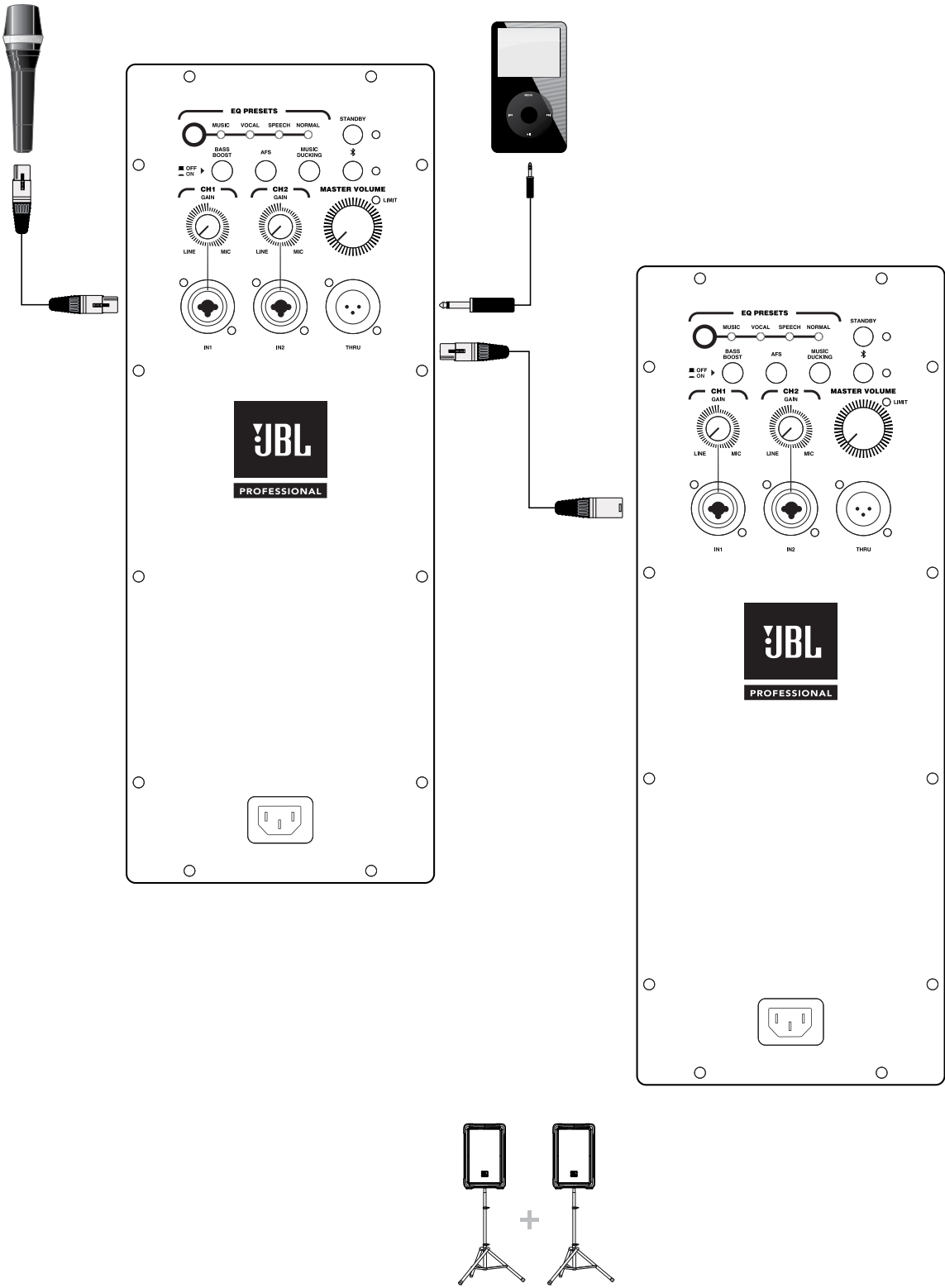
SMALL PA USING BOTH INPUTS AND THRU FUNCTION CH1 input set to "Mic" CH2 input set to "Line" Main Speaker Position
