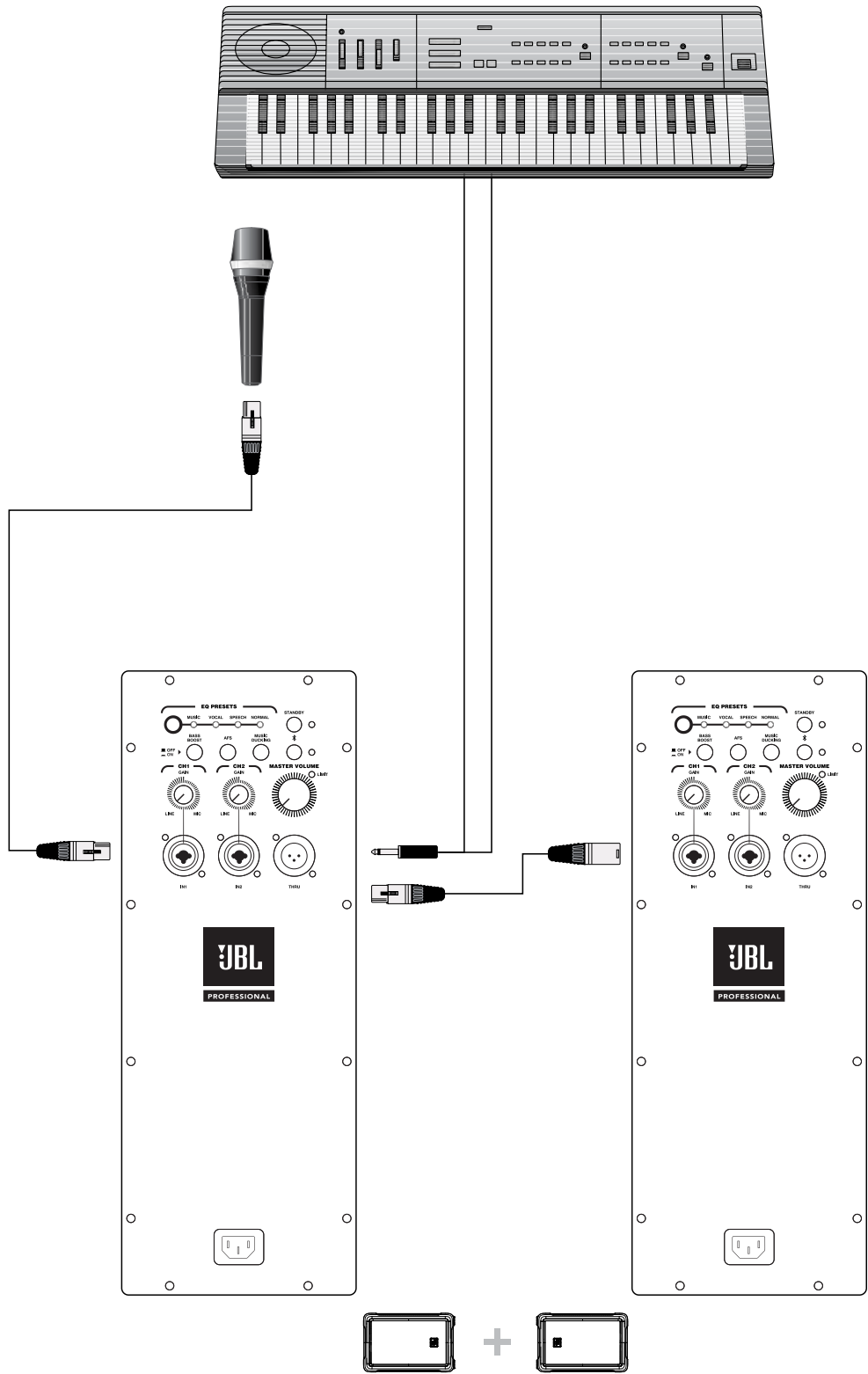
SMALL PA USING TWO SYSTEMS AS MONITORS CH1 input set to “Mic” CH2 input set to “Line” Monitor Speaker Position
