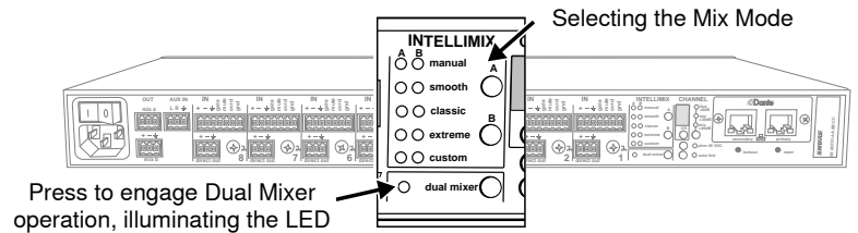
Back Panel
