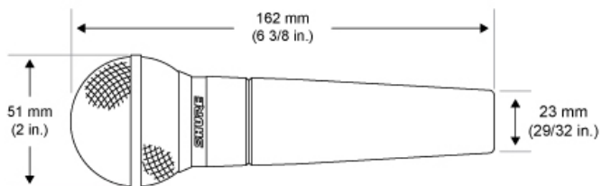
Overall Dimensions
