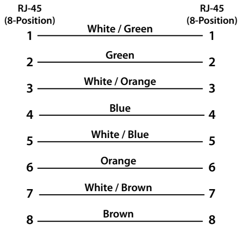
TIA/EIA 568A Straight-Through
