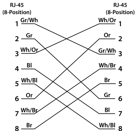
TIA/EIA 568A Crossover
