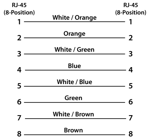
TIA/EIA 568B Straight-Through
