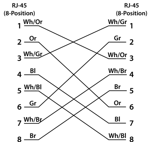
TIA/EIA 568B Crossover
